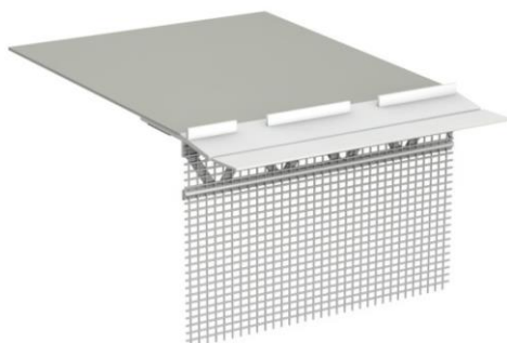
sl. 1: StoFentra Guard kotnik in srednji kos
